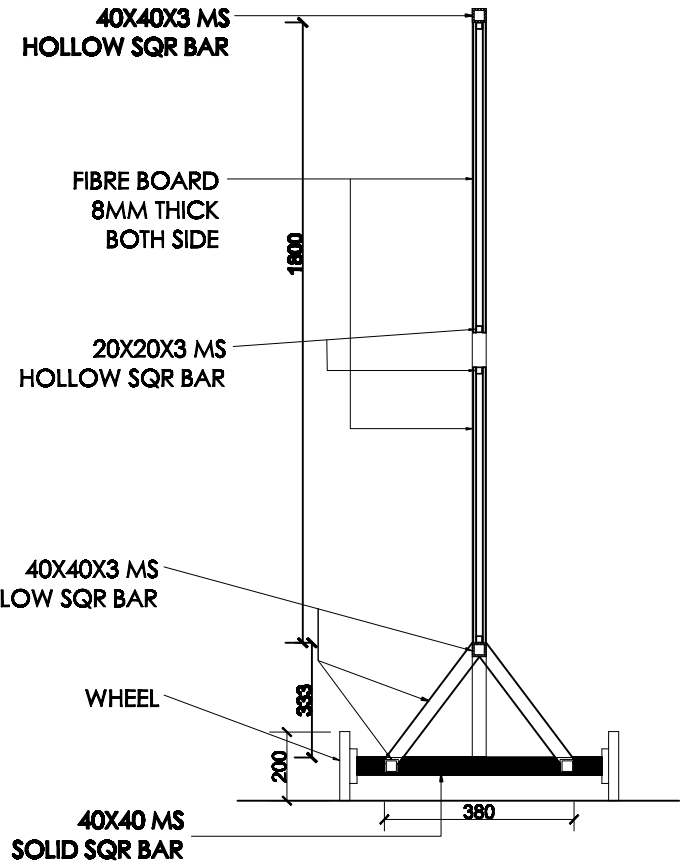
SEC X-X 1:25
